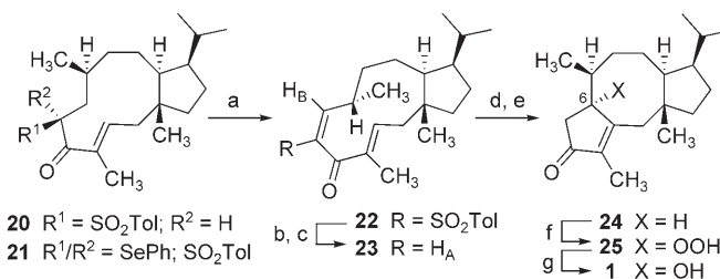
Scheme 4. Reagents and conditions: a) \text{NaHMDS} , \text{THF} , -78^\circ\text{C} , \text{PhSeCl} , 0^\circ\text{C} , then aq. \text{H}_2\text{O}_2 , 98%; b) \text{DIBAL} , -78^\circ\text{C} , 95%; c) sodium naphthalide, \text{THF} , -78^\circ\text{C} , 1 min, then \text{MnO}_2 , \text{PhH} , 70%; d) \text{TsOH} (cat.), \text{ClCH}_2\text{CH}_2\text{Cl} , 92%; e) t\text{BuOCl} , aq. acetone, 40%; f) air oxidation; g) \text{CH}_2\text{Cl}_2 , aq. \text{NaHSO}_3 (95%). \text{HMDS} = 1,1,1,3,3,3 -hexamethyl-disilazane.
